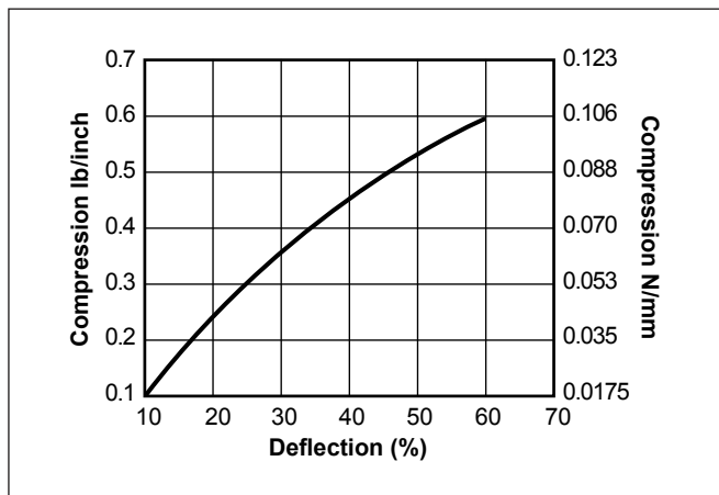
Figure 1 Typical Compression-Deflection
